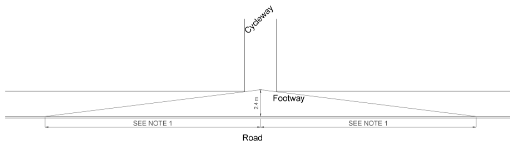
Figure DG10 Visibility plays at junctions for cyclists
